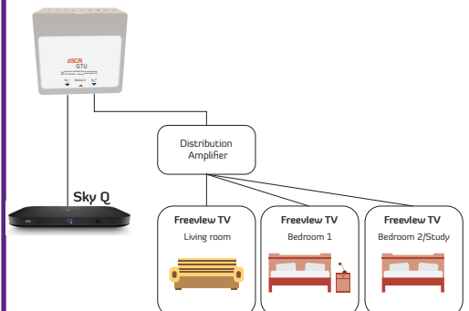
Diagram 2 Sky Q with a 'Distribution Amplifier'
